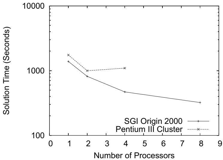
FIGURE 9: Comparison of the Performance of MPI on the Origin 2000 and a Beowulf Cluster
