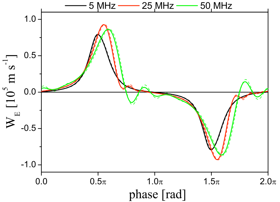
FIGURE 2: Comparison of the Boltzmann (solid) and Monte Carlo (dashed) results for W_E over a range of applied frequencies for the Reid ramp model.
